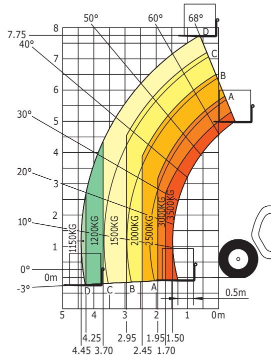
Machine with forks on tyres
